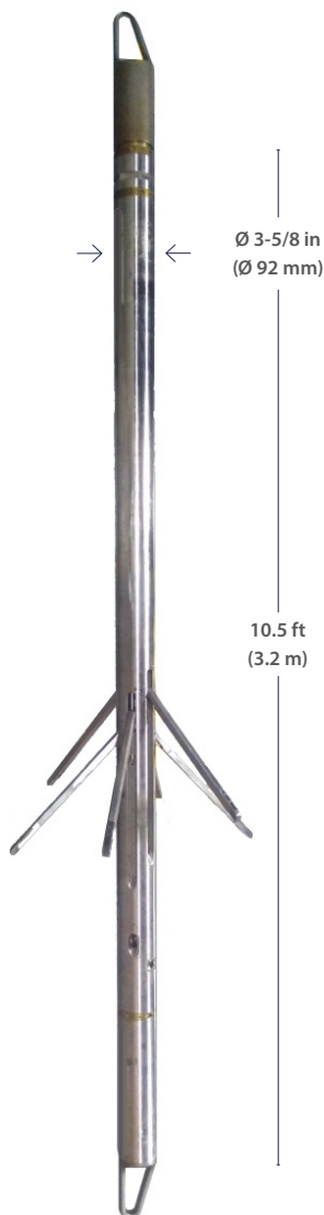
SIX-ARM CALIPER
